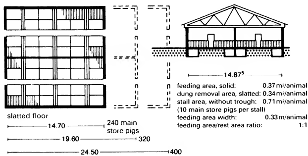
④ Store pig shed: four rows, central wall, long stalls, transverse troughs
